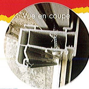
3 Vissage direct auto-perceuse
