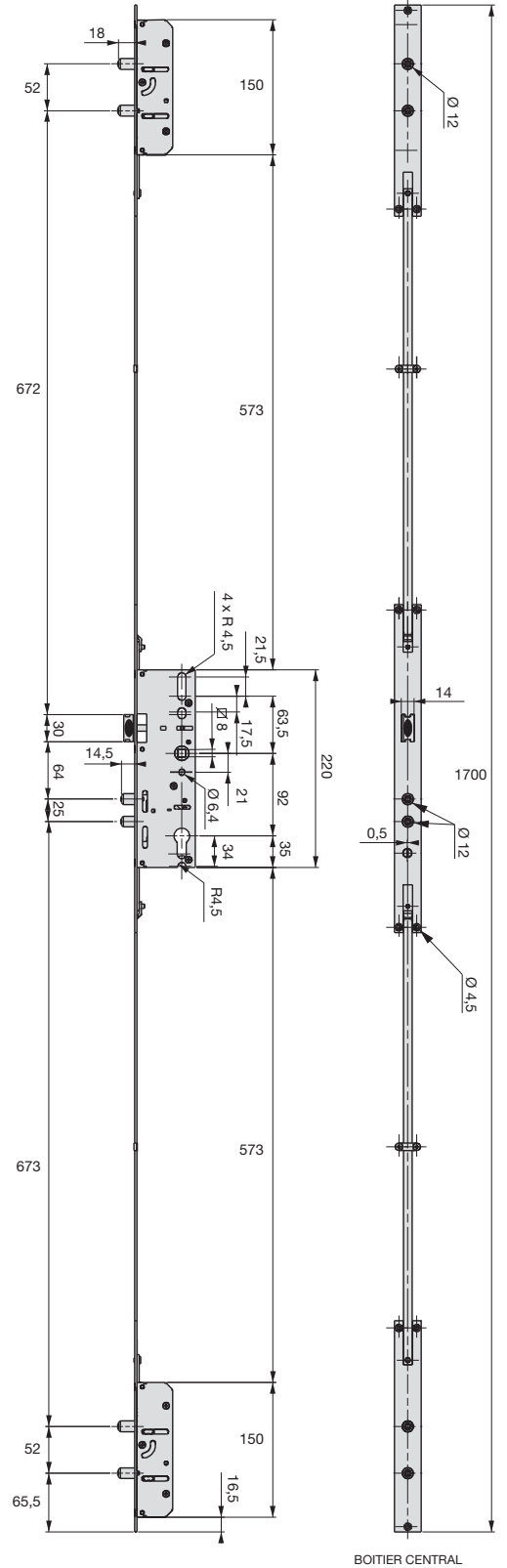
BOITIER CENTRAL
