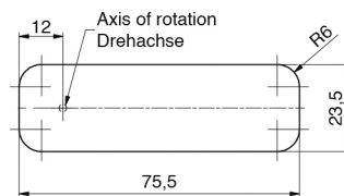
Stamping configuration Stanzbild
