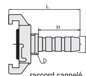
raccord cannelé
