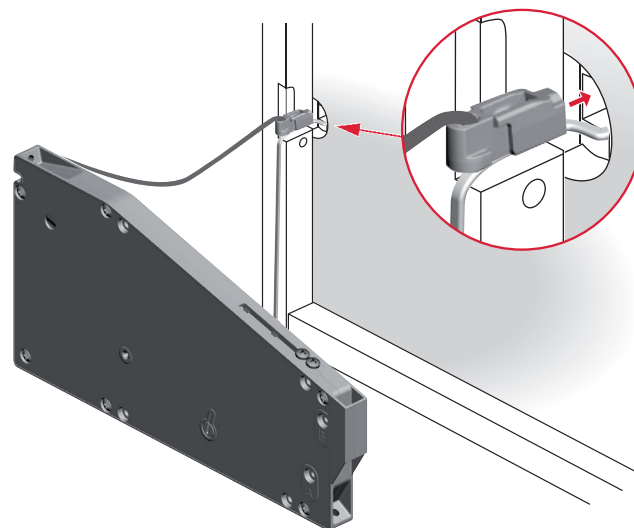
WIRE INSTALLATION
