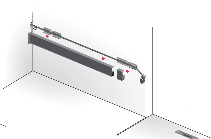
COVER CAPS AND ALUMINIUM LATERAL PROFILE INSERTION
