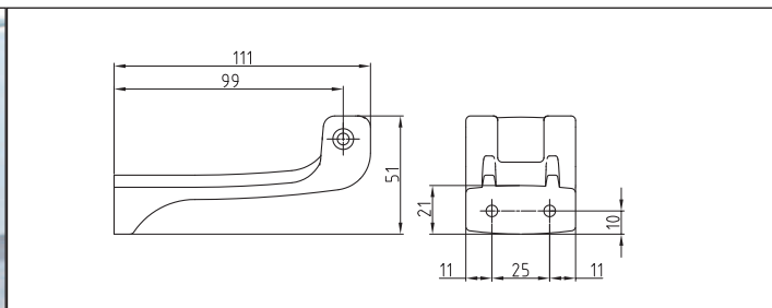
Grey: Part No. 41582C Black: Part No. 41583D White: Part No. 41584E
